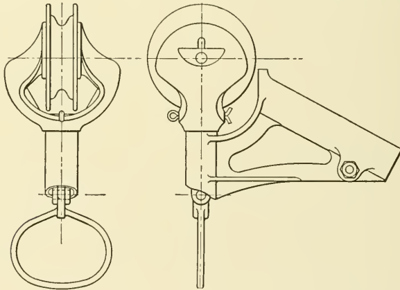
Fig. 15. Views of Trolley Pulley Showing Ring by Which Trolley Is Shifted
